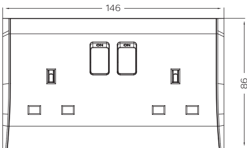
Dimensions for 2gang frames
