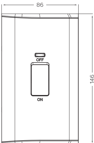
Dimensions for 1gang 45A DP switch (6x3)
