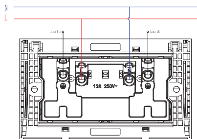
2G switched multi socket
