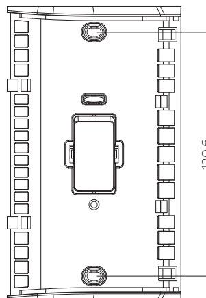
Distance between fixing screws for 45A DP switch (6x3)
