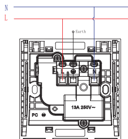
1G switched multi socket
