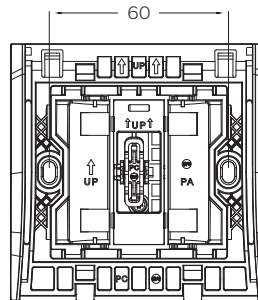
Distance between fixing screws for 1gang frames
