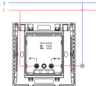
Sensor switch
