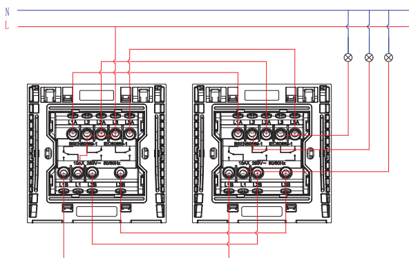
3G 2W switch
