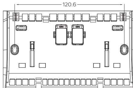
Distance between fixing screws for 2gang frames
