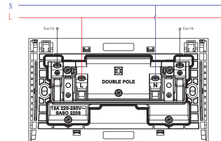
2G 13A switched socket DP
