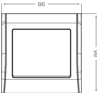
Dimensions for 1gang frames
