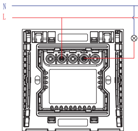
1G dimmer switch (250W)
