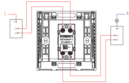
1G intermediate switch
