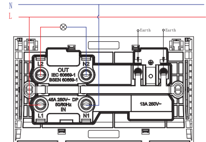
Cooker control unit
