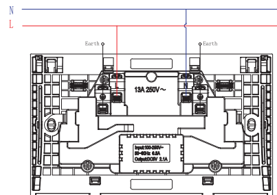
2G switched multi socket + 2*USB
