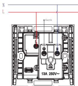
1G 13A switched multi socket + 1*USB
